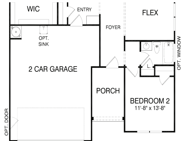
First Floor Plan w/ Opt. 4'-0" Garage Extension
