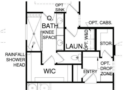
Owner's Bath Option 3
