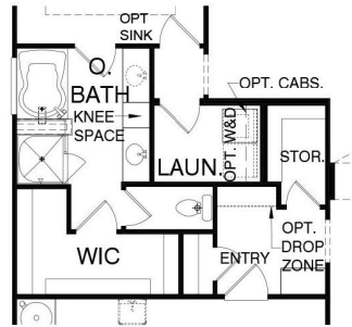
Owner's Bath Option 2
