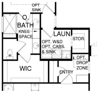
Owner's Bath Option 1
