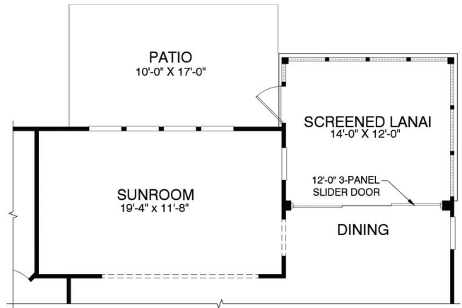
First Floor Plan w/ Opt Rear Entry Door 4 @ Sunroom w/ Screened Lanai
