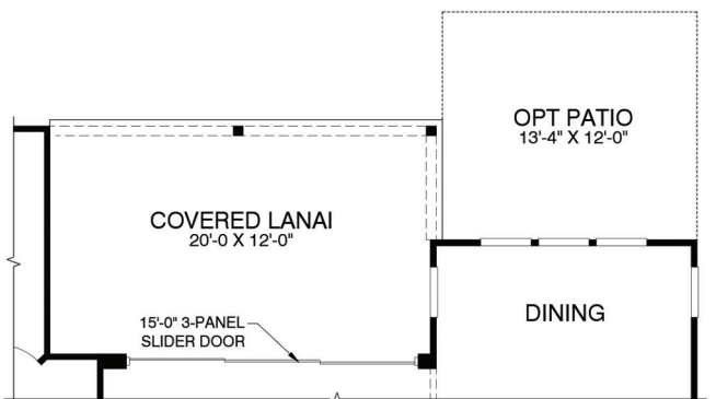
First Floor Plan w/ Opt Rear Entry Door 4 @ Covered Lanai
