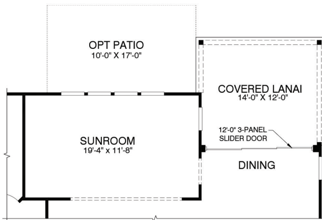
First Floor Plan w/ Opt Rear Entry Door 4 @ Sunroom w/ Covered Lanai
