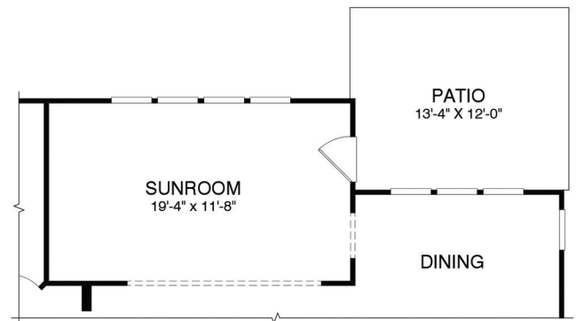
First Floor Plan w/ Opt Sunroom
