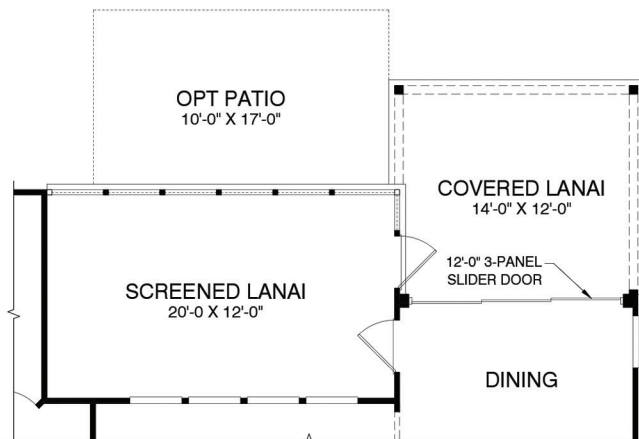
First Floor Plan w/ Opt Rear Entry Door 4 @ Screened Lanai w/ Covered Lanai
