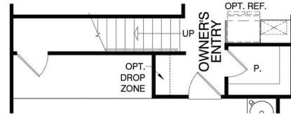
First Floor Plan w/ Opt. Loft Stairs
