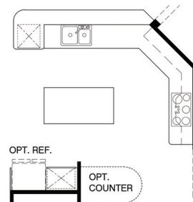
Cabinets for Built-In Appliances w/ Stagger Options
