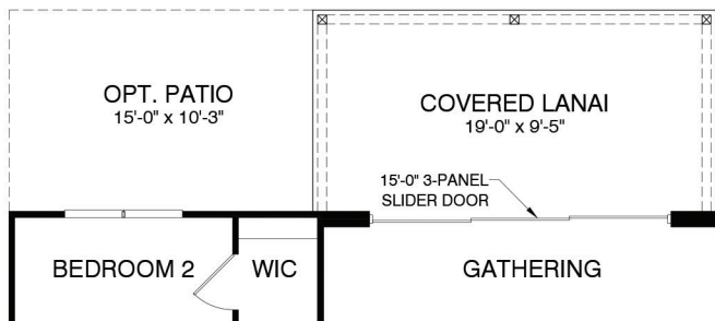
First Floor Plan w/ Opt. Rear Entry Door 4 @ Covered Lanai
