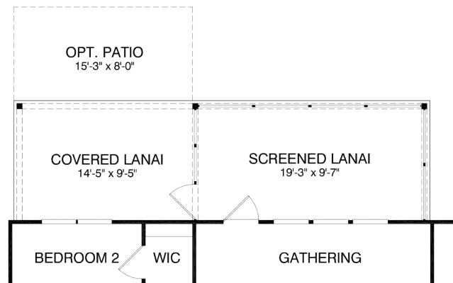
First Floor Plan w/ Opt. Screened Lanai & Covered Lanai
