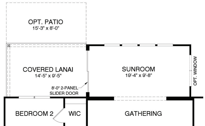
First Floor Plan w/ Opt. Rear Entry Door 4 @ Sunroom w/ Covered Lanai
