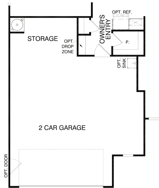
First Floor Plan w/ Opt. 4'-0" Garage Extension
