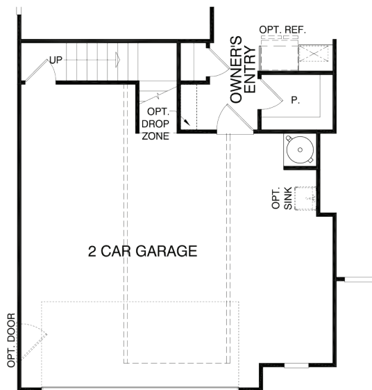
First Floor Plan w/ Opt. Garage Attic Storage & 4'-0" Garage Extension
