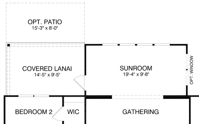
First Floor Plan w/ Opt. Sunroom & Covered Lanai
